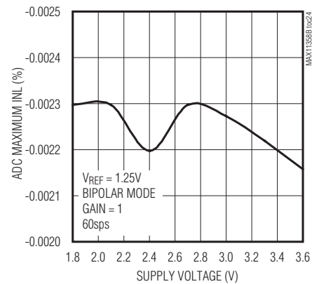
ADC MAXIMUM INL vs. SUPPLY VOLTAGE
