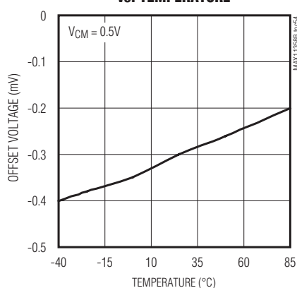
OP-AMP INPUT OFFSET VOLTAGE vs. TEMPERATURE
