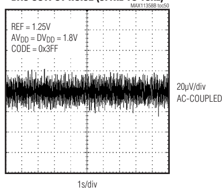
DAC OUTPUT NOISE (0.1Hz TO 10Hz)
