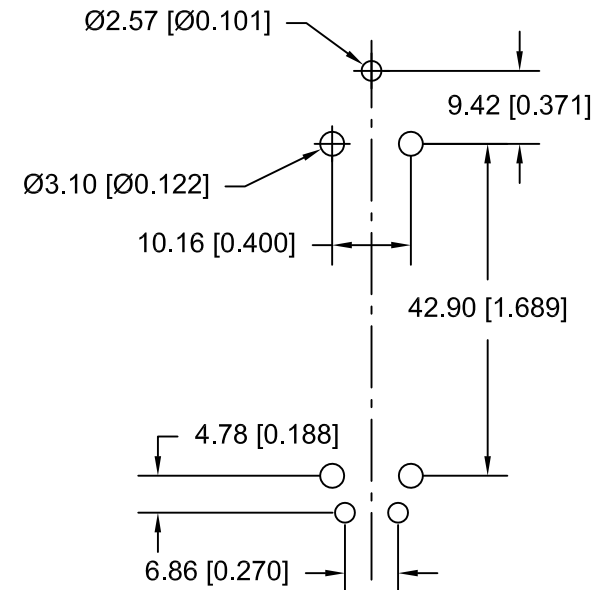
PCB LAYOUT
