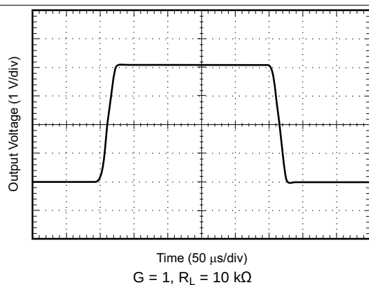
Figure 9. Large-Signal Step Response
