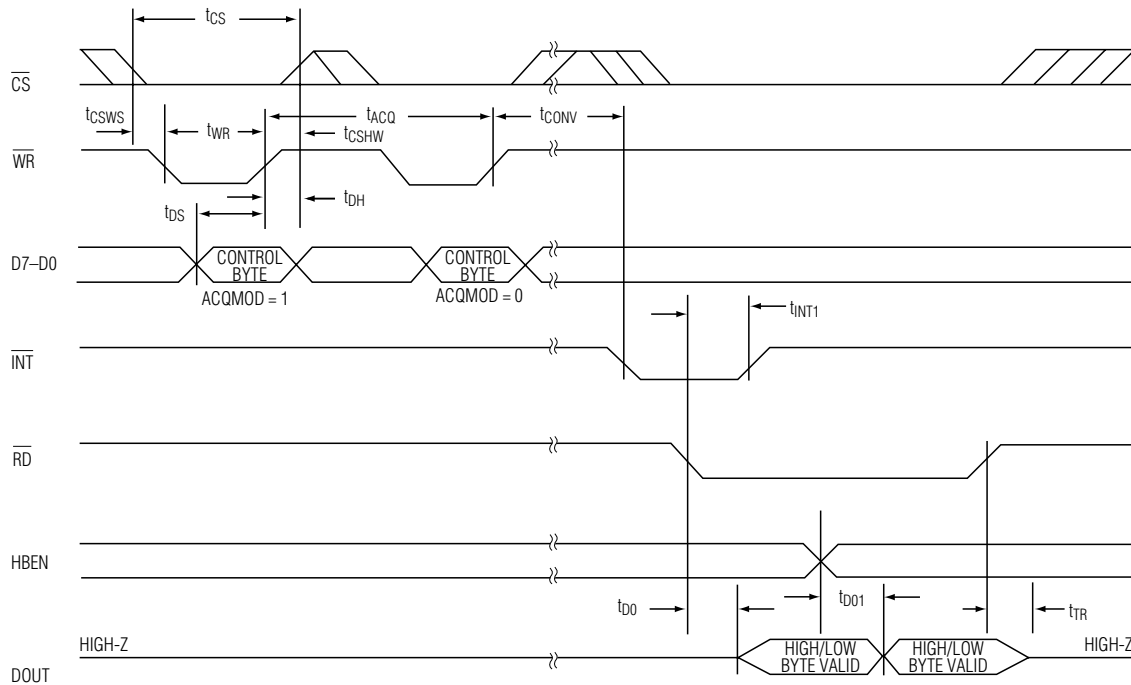
Figure 5. Conversion Timing Using External Acquisition Mode
