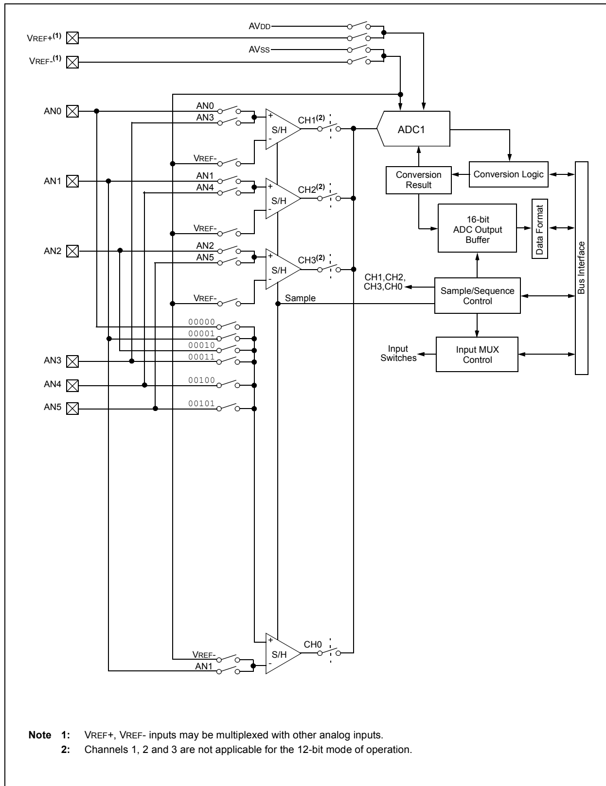
FIGURE 19-2: ADC1 MODULE BLOCK DIAGRAM FOR dsPIC33FJ32MC202 DEVICES
