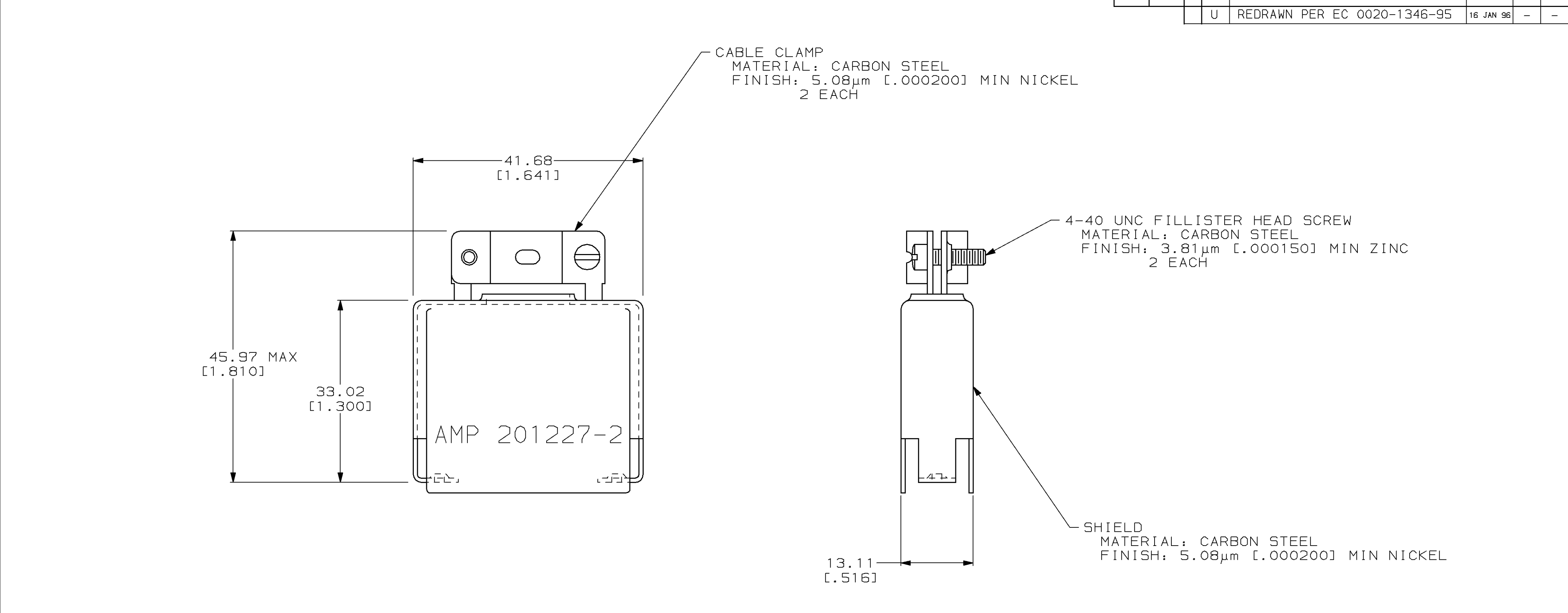
ASSEMBLED VIEW
