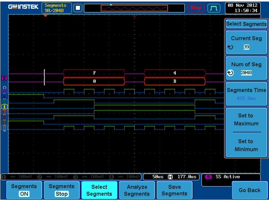
Figure 4: The Implement Result of Segmented Memory Function.
