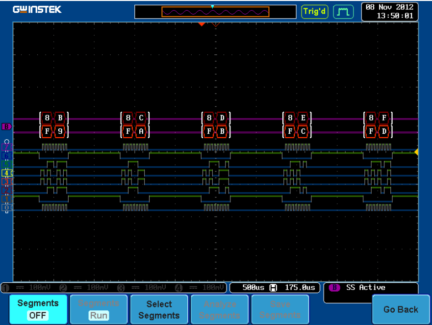
Figure 3: How to Implement Segmented Memory Function on GDS-2000A
