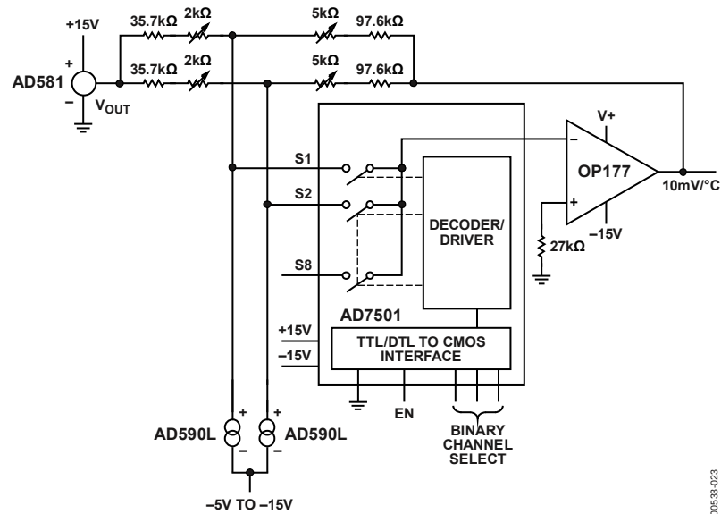
Figure 24. 8-Channel Multiplexer
