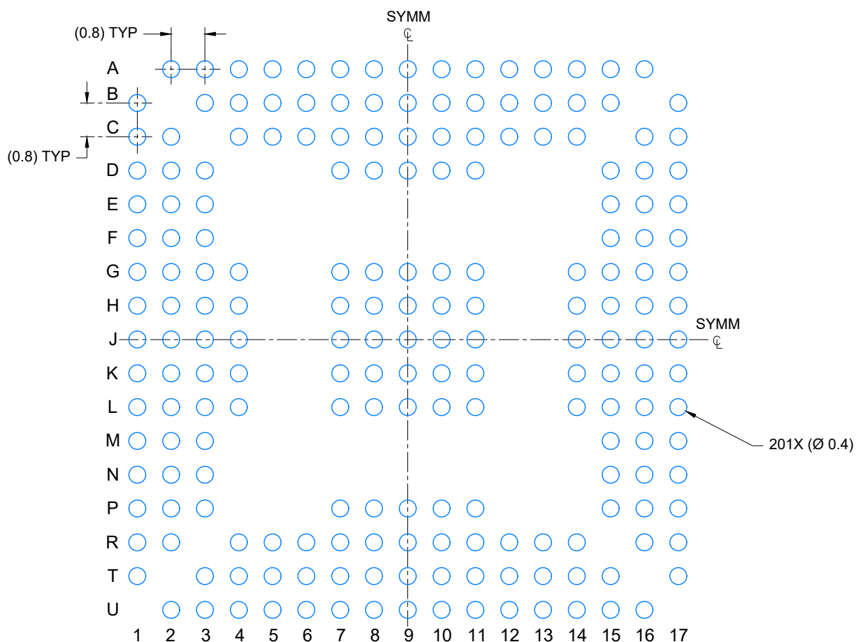
LAND PATTERN EXAMPLE
