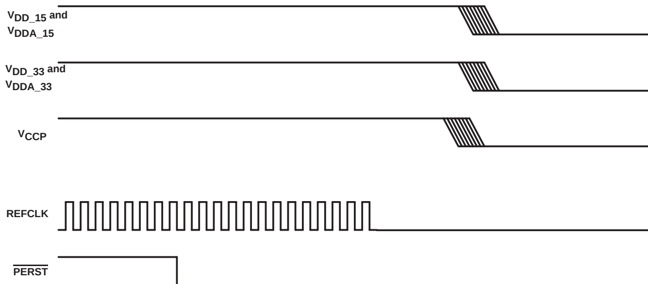
Figure 3–3. Power-Down Sequence
