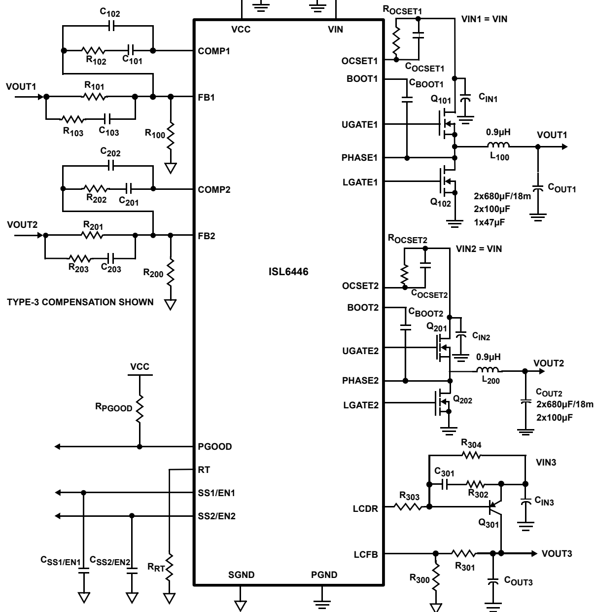
FIGURE 4. ISL6446 TYPICAL APPLICATION
