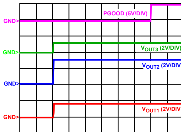
FIGURE 21. PGOOD DELAY
