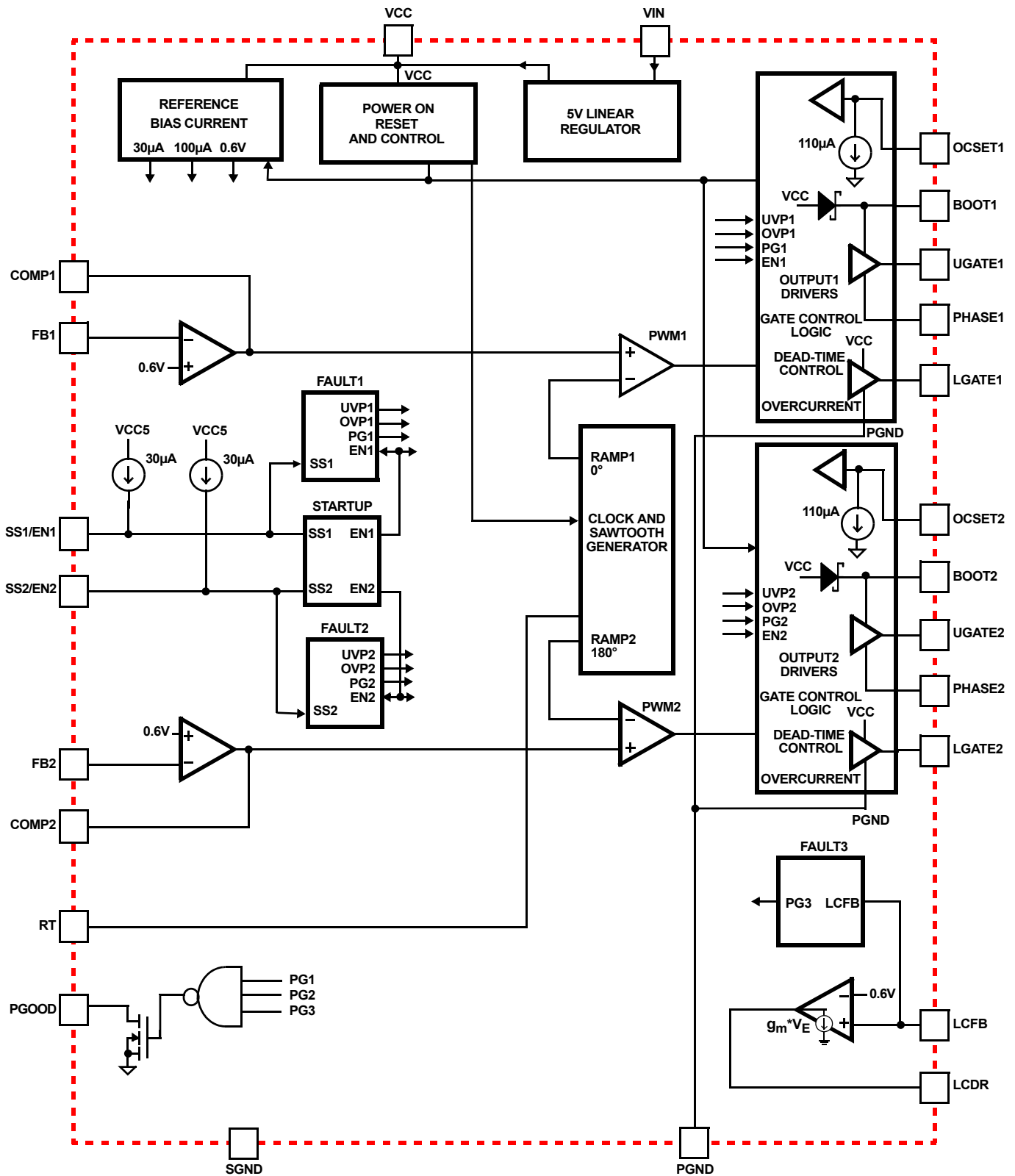
FIGURE 3. BLOCK DIAGRAM
