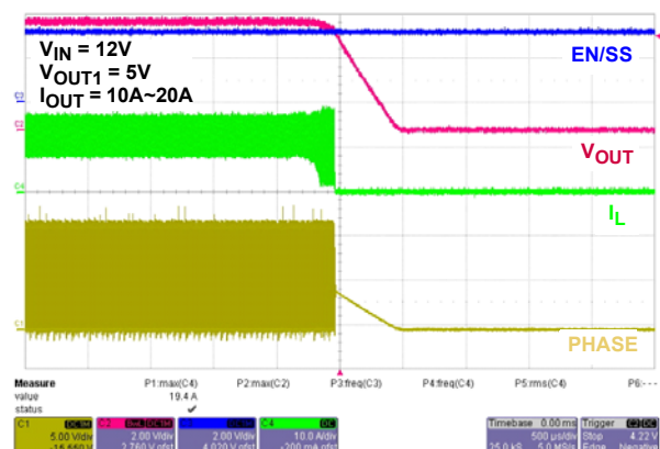
FIGURE 15. OVERCURRENT PROTECTION
