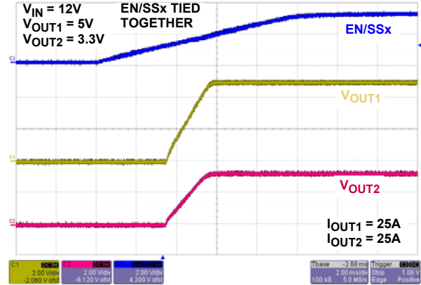
FIGURE 11. EN/SS START-UP
