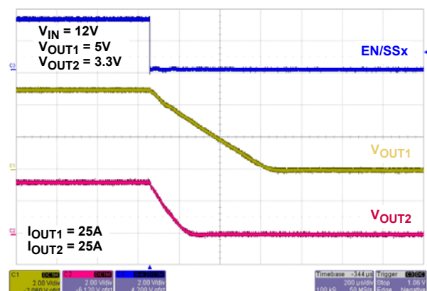
FIGURE 13. EN/SS SHUT-DOWN
