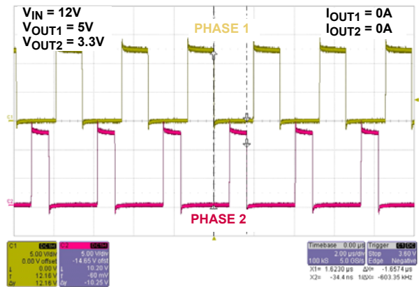
FIGURE 8. PWM INTERLEAVING
