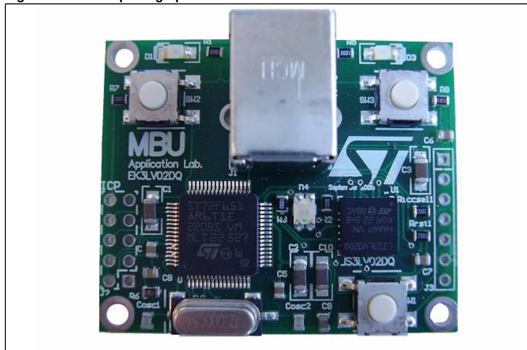
Figure 3. Board photograph
