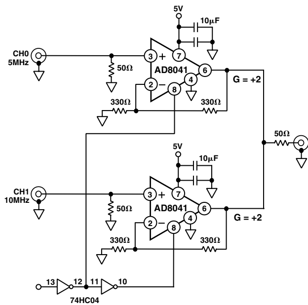
Figure 7. 2:1 Multiplexer
