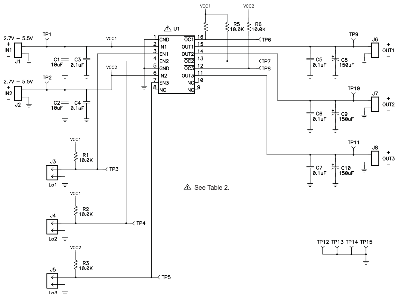
Figure 1. TPS20xxEVM-294 Schematic
