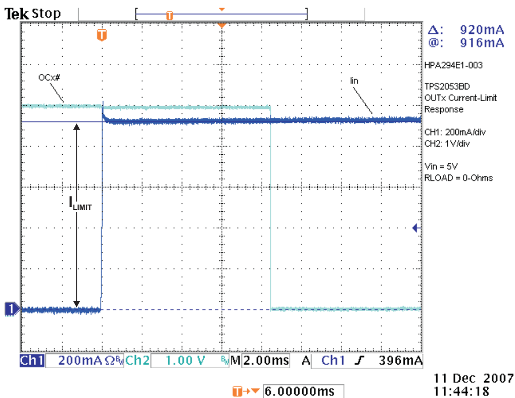
Figure 3. TPS2053BEVM-294 Short-Circuit Output Current and \overline{OCx} Status
