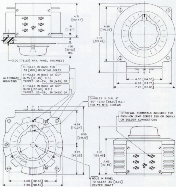
PANEL MOUNTED
