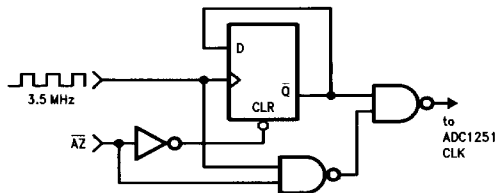
FIGURE 5. Switching between a Conversion with and without Auto-Zero when Using \overline{WR} Control
