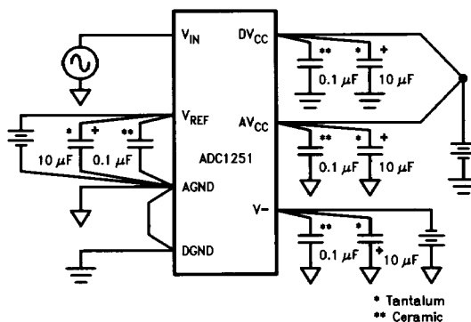
Power Supply Bypassing
