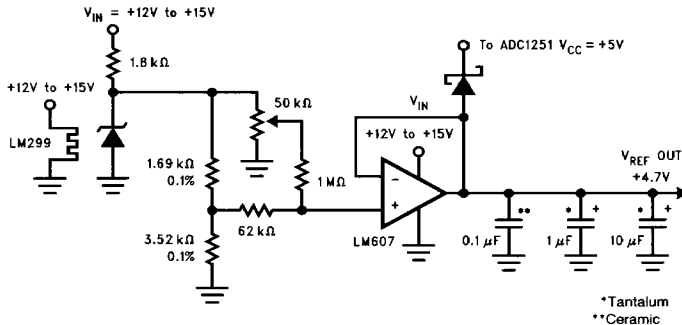
FIGURE 4. Low Drift Extremely Stable Reference Circuit
