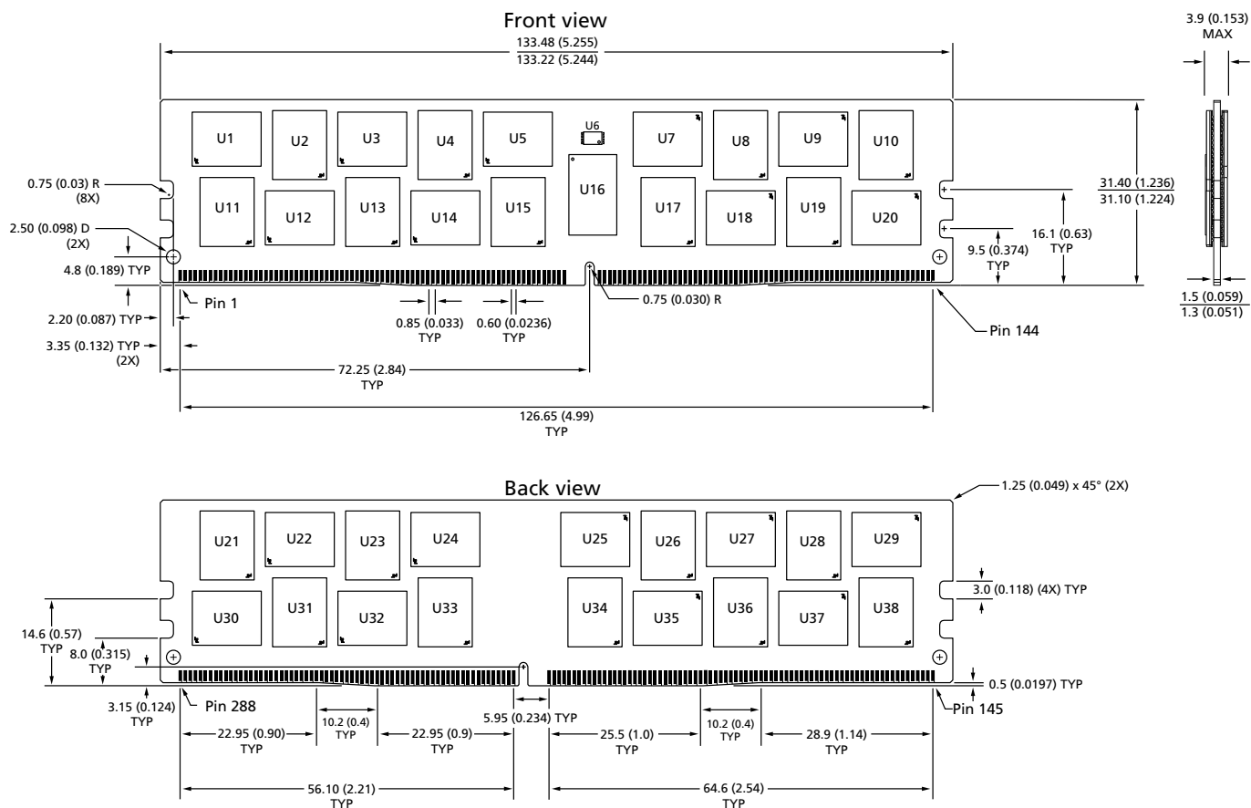
Figure 7: 288-Pin DDR4 RDIMM (R/C-B, PCB 1506)
