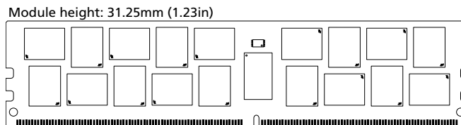
Figure 2: 288-Pin RDIMM (MO-309, R/C-B1)
