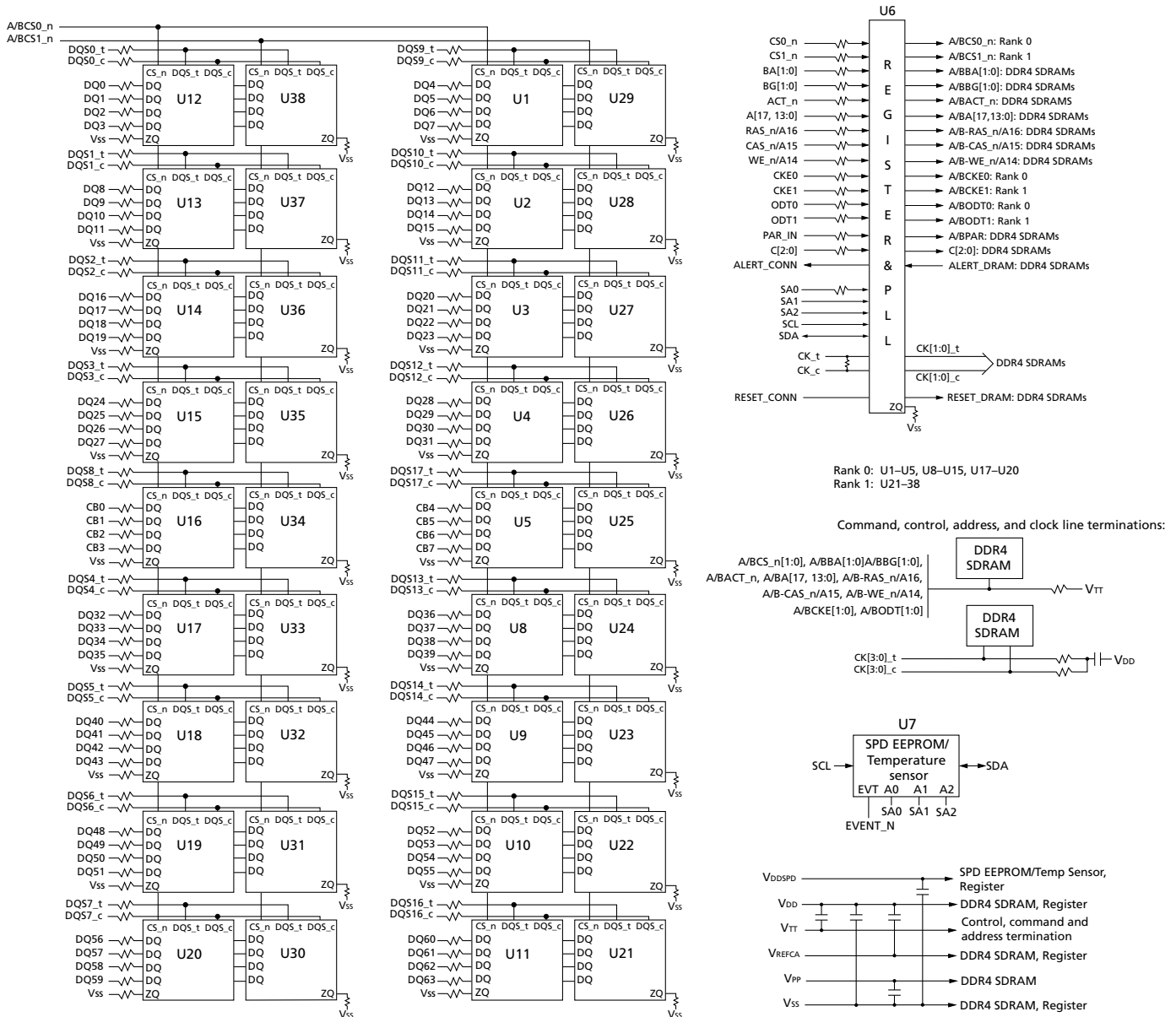
Figure 5: Functional Block Diagram (R/C-B1, PCB 1798, PCB 1870)
