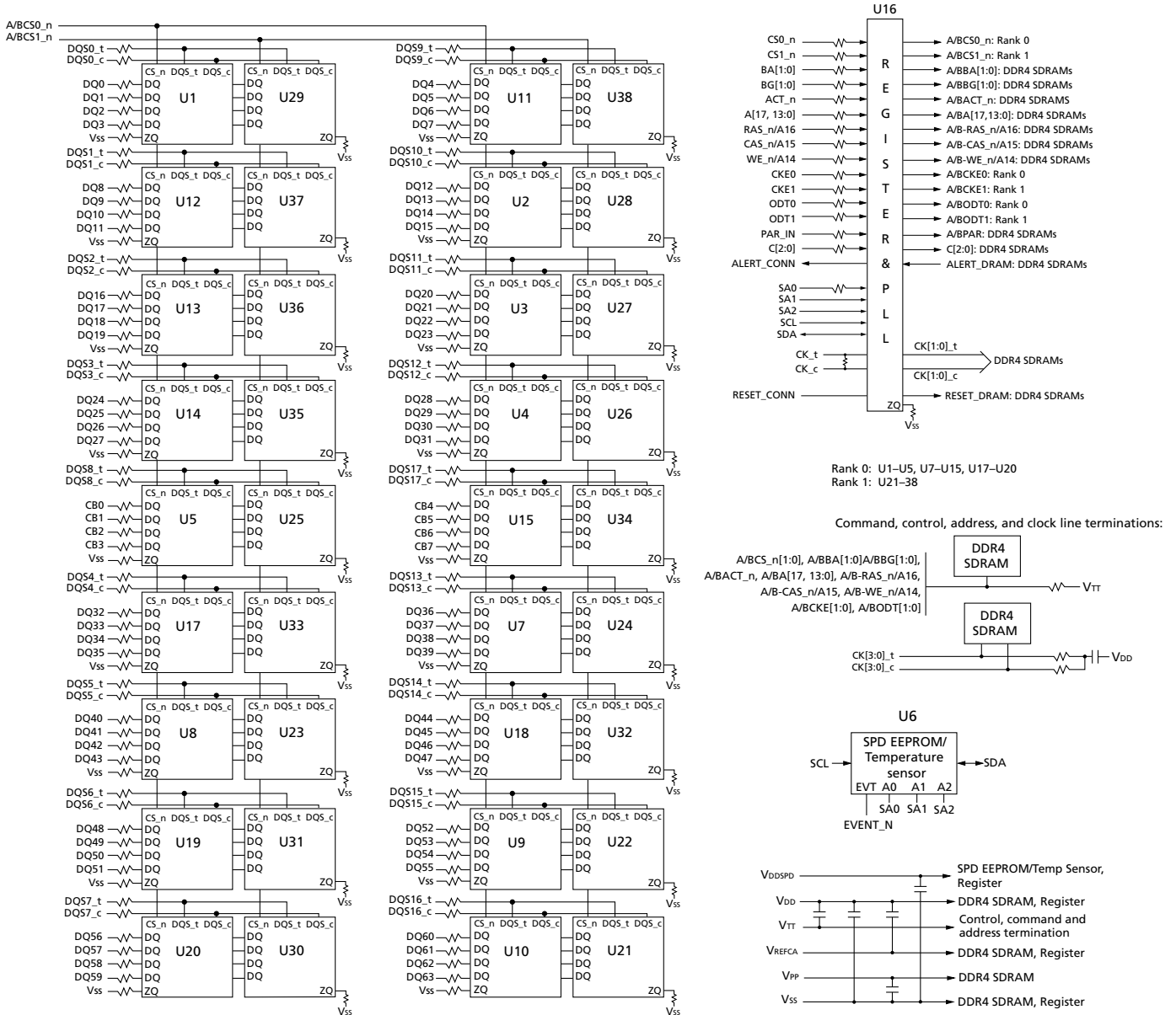
Figure 4: Functional Block Diagram (R/C-B, PCB 1506)
