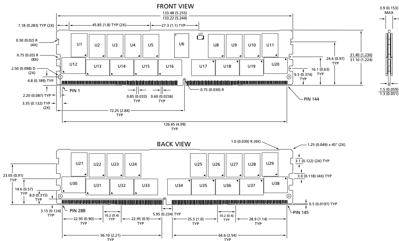
Figure 8: 288-Pin DDR4 RDIMM (R/C-B1, PCB 1798, PCB 1870)
