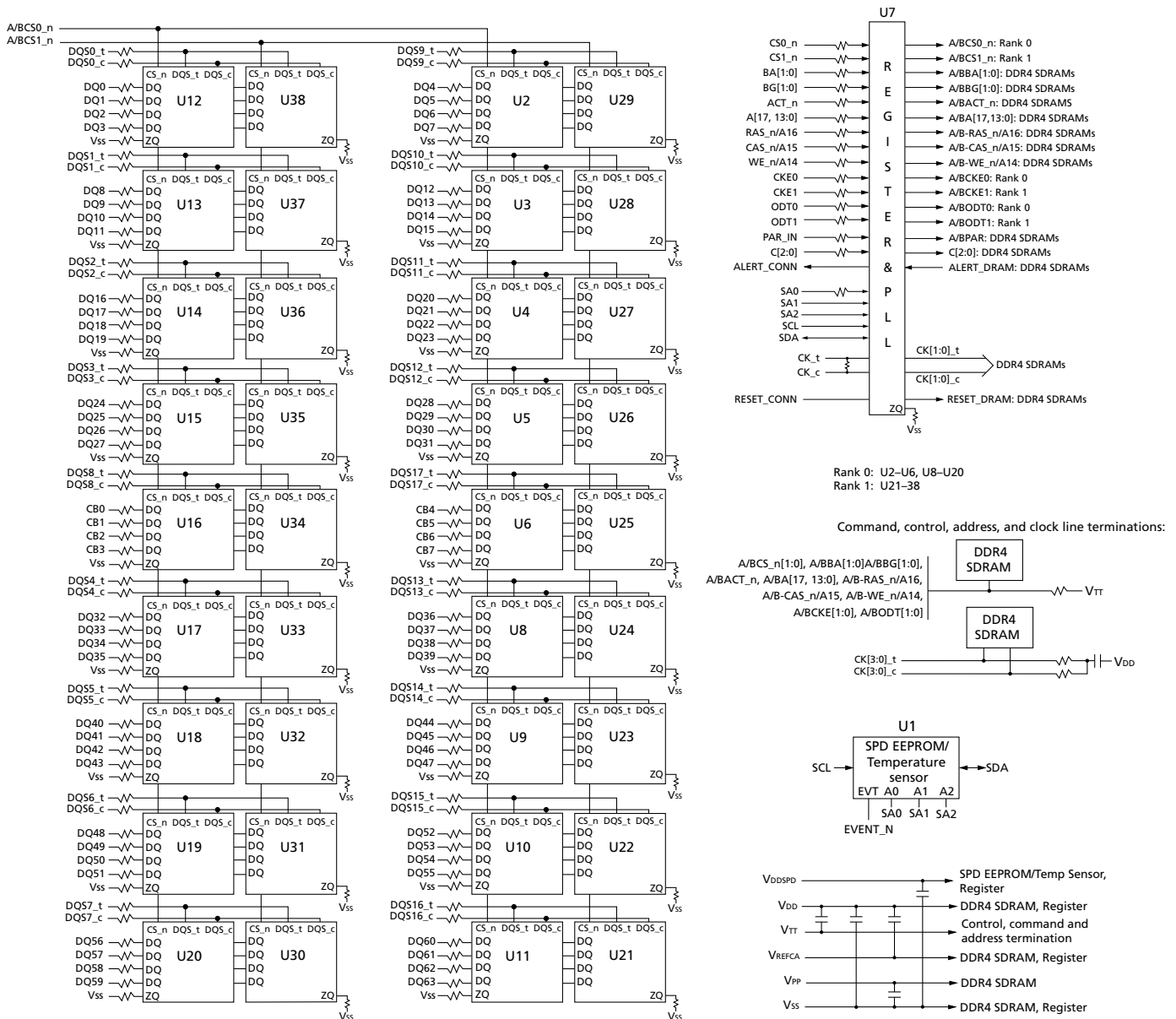
Figure 6: Functional Block Diagram (R/C-B2, PCB 2364)
