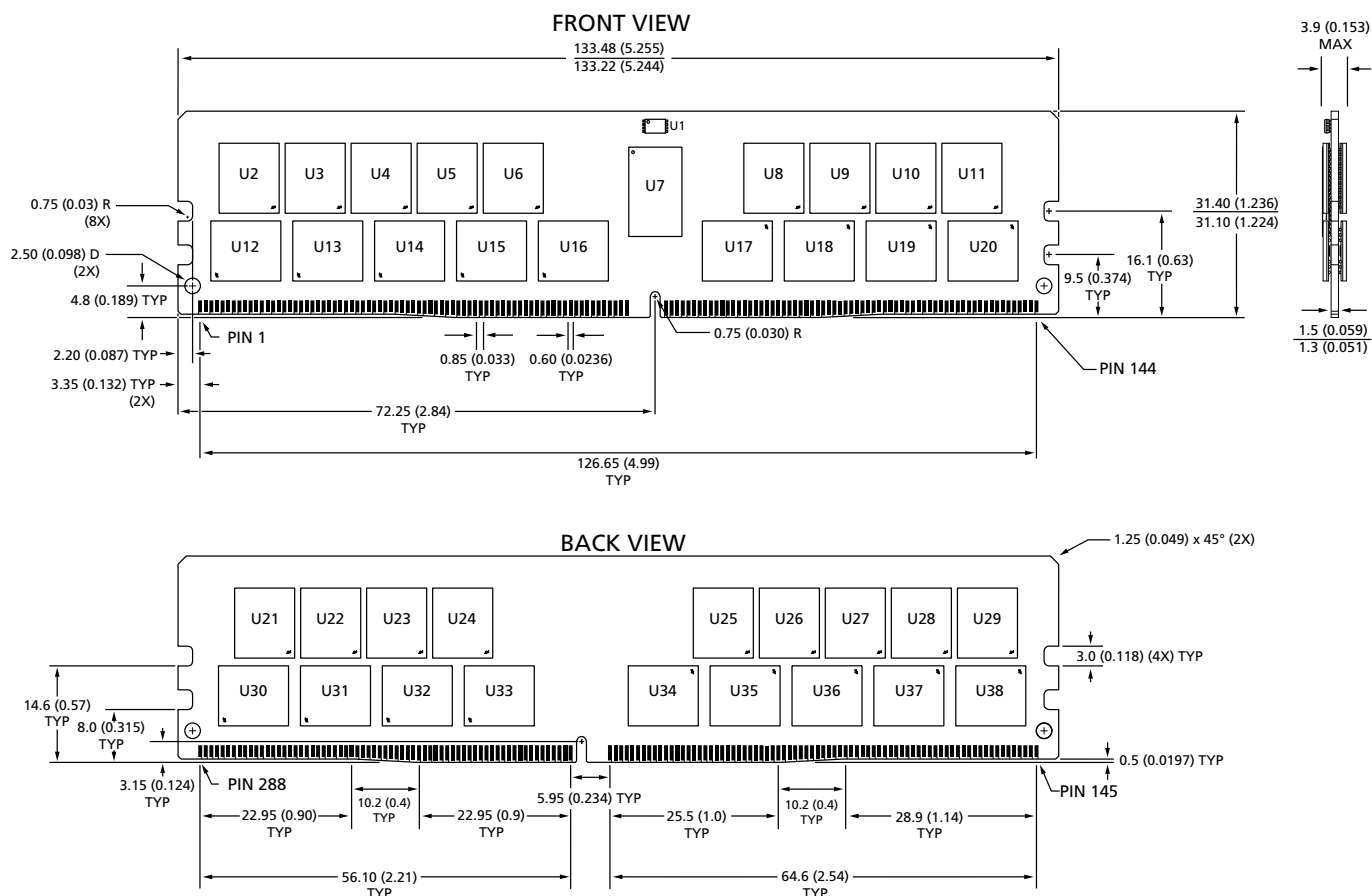
Figure 9: 288-Pin DDR4 RDIMM (R/C-B2, PCB 2364)
