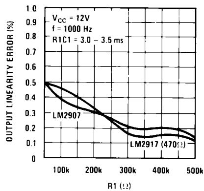
Tachometer Linearity vs R1
