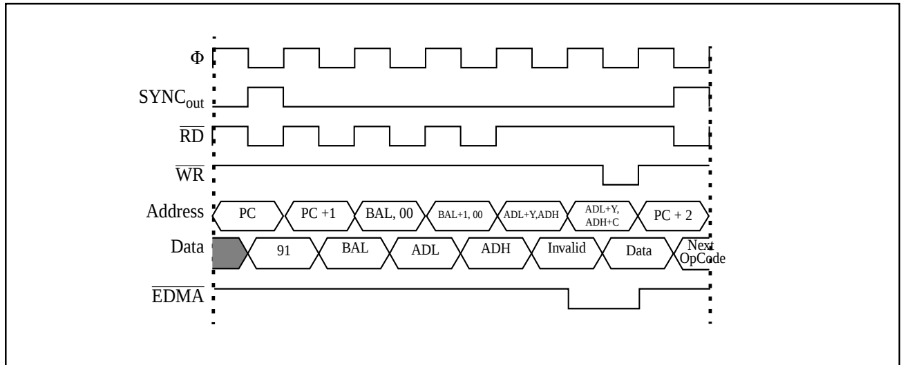
Fig. 1.13. Instruction sequences for STA ($zz) IndY with \text{EDMA} Enable
