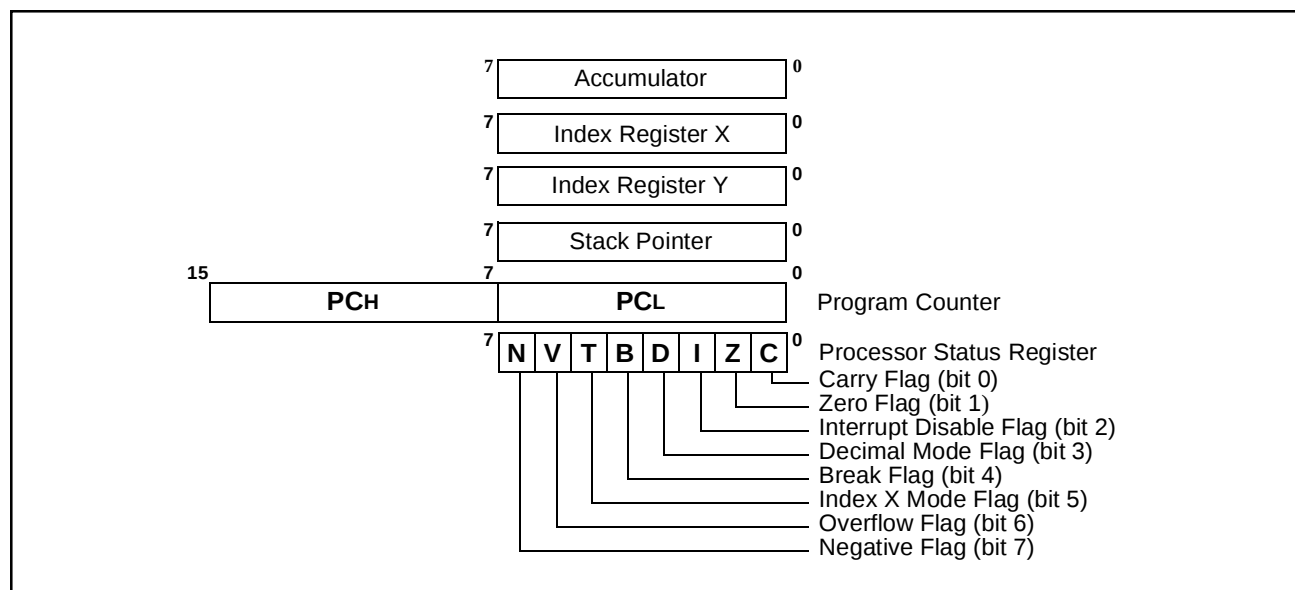
Fig. 1.4. Register Structure
