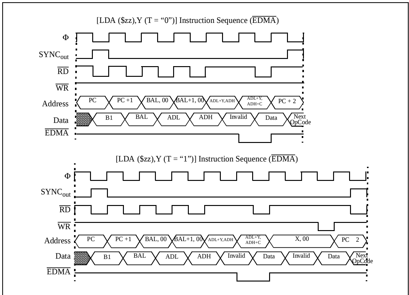
Fig. 1.14. Instruction sequences for LDA ($zz) IndY with \text{EDMA} Enable
