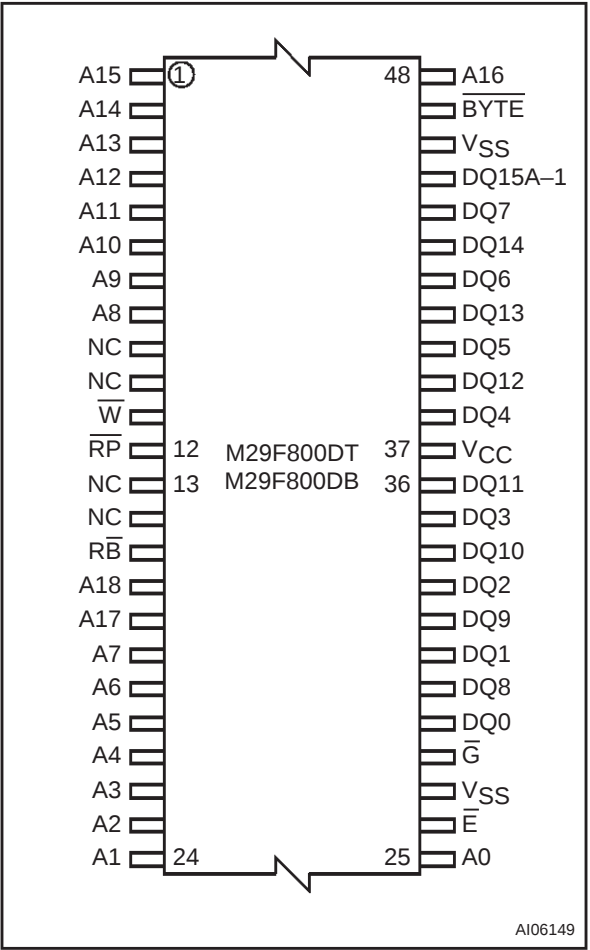
Figure 4. TSOP Connections
