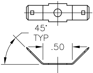
ITEM #2 - CAT NO. QC-21 TOP HARDWARE CODE - 21
