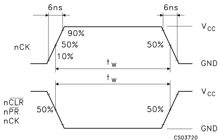
Figure 8: Waveform - Minimum Pulse Width ( \overline{nCLR} , \overline{nPR} , nCK ) ( f=1\text{MHz} ; 50% duty cycle)
