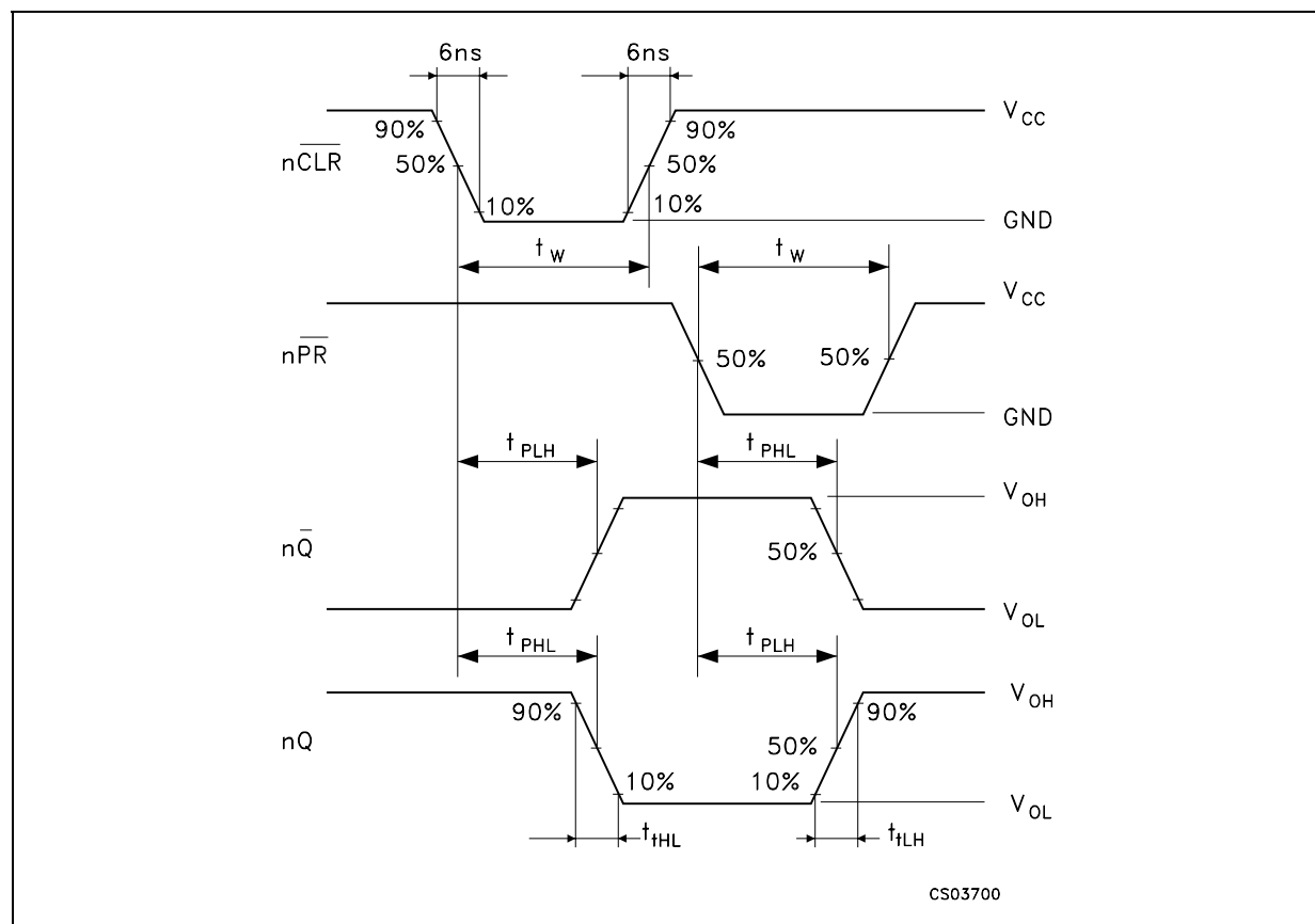
Figure 7: Waveform - Minimum Pulse Width ( n\overline{CLR} and n\overline{PR} ), Minimum Removal Time ( n\overline{CLR} and n\overline{PR} TO nCK ) ( f=1\text{MHz} ; 50% duty cycle)
