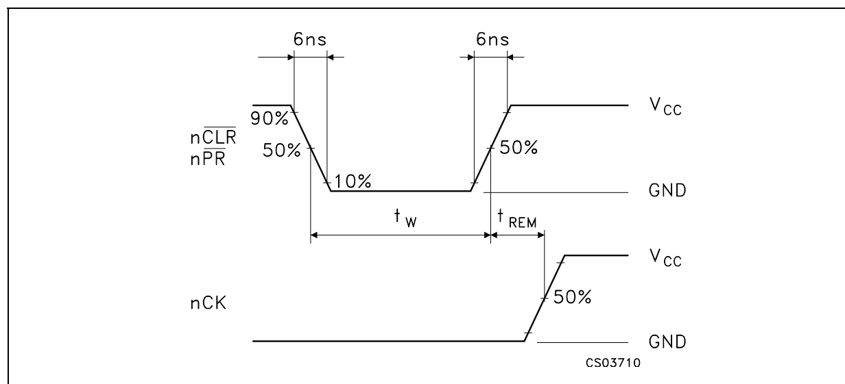
Figure 7: Waveform - Minimum Pulse Width ( n\overline{CLR} and n\overline{PR} ), Minimum Removal Time ( n\overline{CLR} and n\overline{PR} TO nCK ) ( f=1\text{MHz} ; 50% duty cycle)
