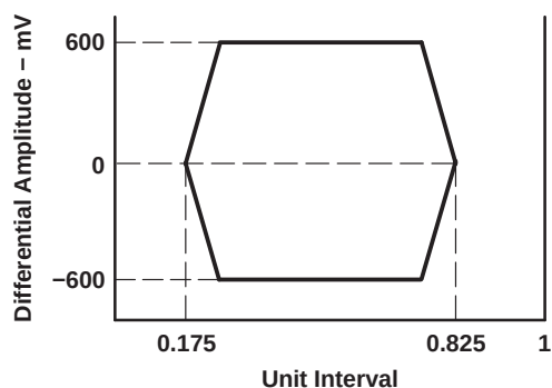
Figure 4-2. Transmit Template
