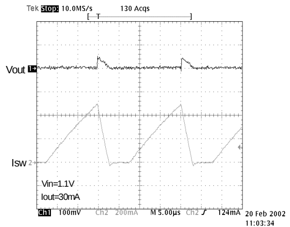
Figure 20 : Switching Waveform
