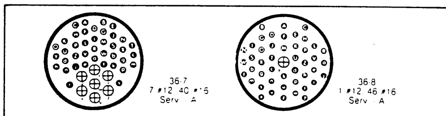
47 contacts
