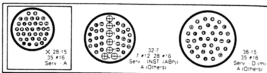
35 contacts
