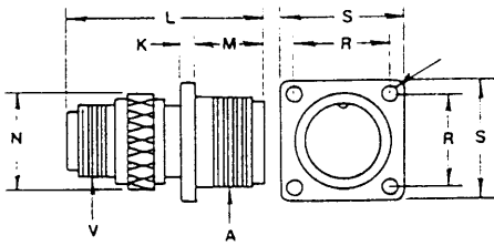
97-4100A/97-4101A
