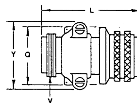
97-4106B straight plug
