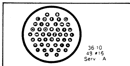
48 contacts
