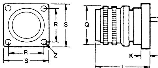
97-5105 construction
