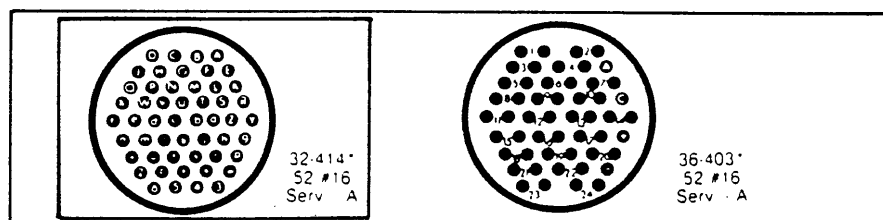
52 contacts
