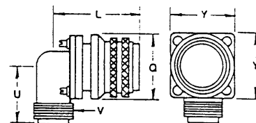
97-4108A angle plug
