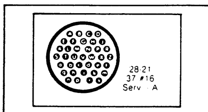
37 contacts
