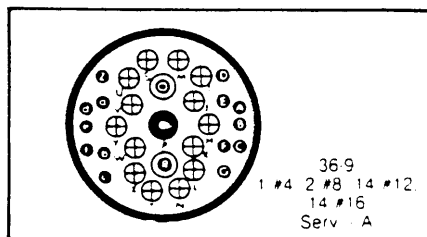
31 contacts
