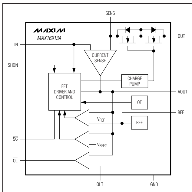
MAX16913A Functional Diagram
