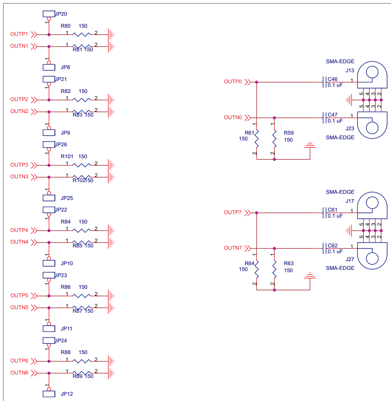
Figure 3. CDCLVP2108EVM—Schematic
