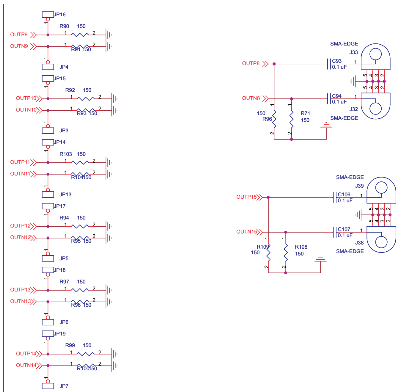
Figure 4. CDCLVP2108EVM—Schematic
