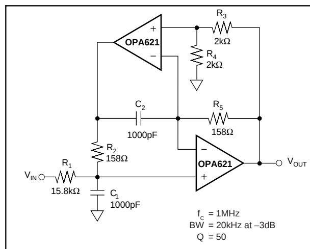
FIGURE 12. High-Q 1MHz Bandpass Filter
