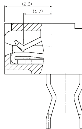
SECT W-W
