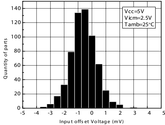
Figure 1: Input offset voltage distribution at T = 25^{\circ}\text{C}
