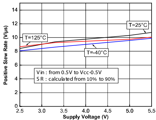
Figure 9: Positive slew rate
