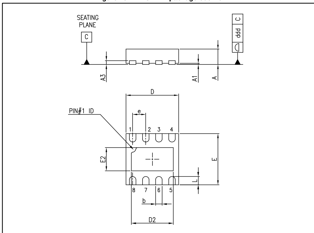
Figure 18: DFN8 2 x 2 package outline
