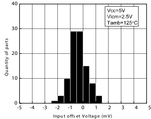
Figure 2: Input offset voltage distribution at T = 125^{\circ}\text{C}
