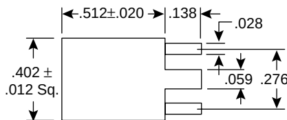
Dimensions (In.)
