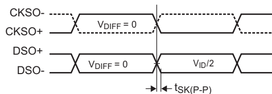
Figure 26. Differential Output Signal Skew
