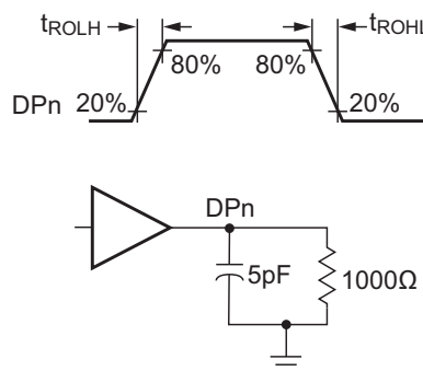
Figure 18. LVCMOS Output Load and Transition Times
