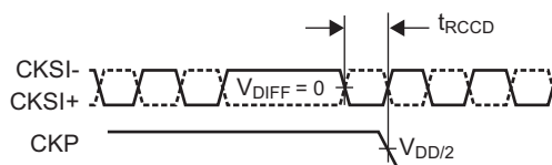
Figure 24. Deserializer Clock Propagation Delay
