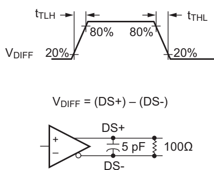
Figure 17. CTL Output Load and Transition Times
