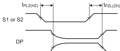
Figure 30. Deserializer Enable and Disable Times
