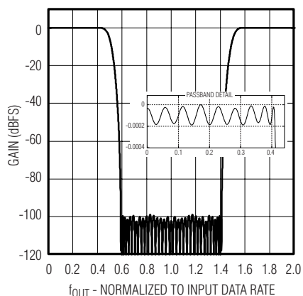
Figure 5. Interpolation Filter Frequency Response, 2x Interpolation Mode
