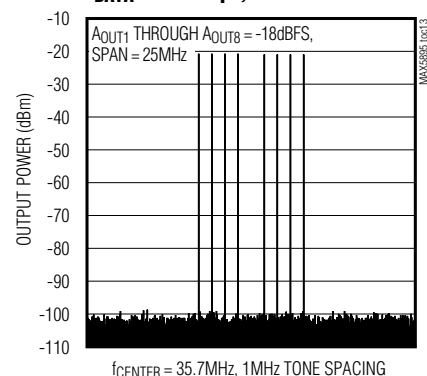
MULTITONE POWER RATIO PLOT f_{DATA} = 125MWps , 2x INTERPOLATION
