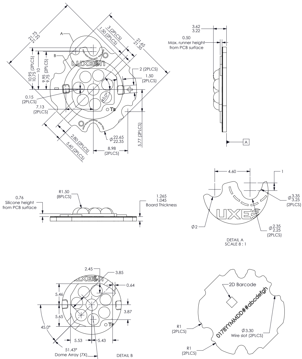
Figure 4. Dimensions for LKx-Pxxx-xxx8(A).
