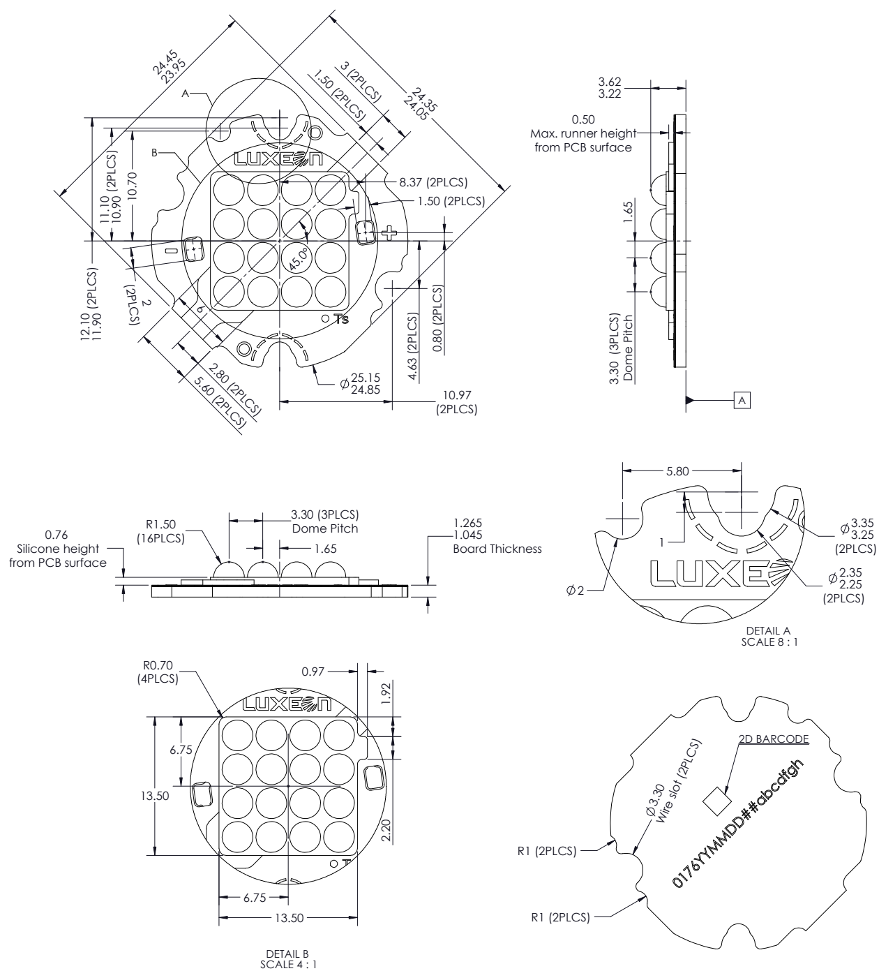
Figure 6. Dimensions for LKx-Pxxx-xx16(A).
