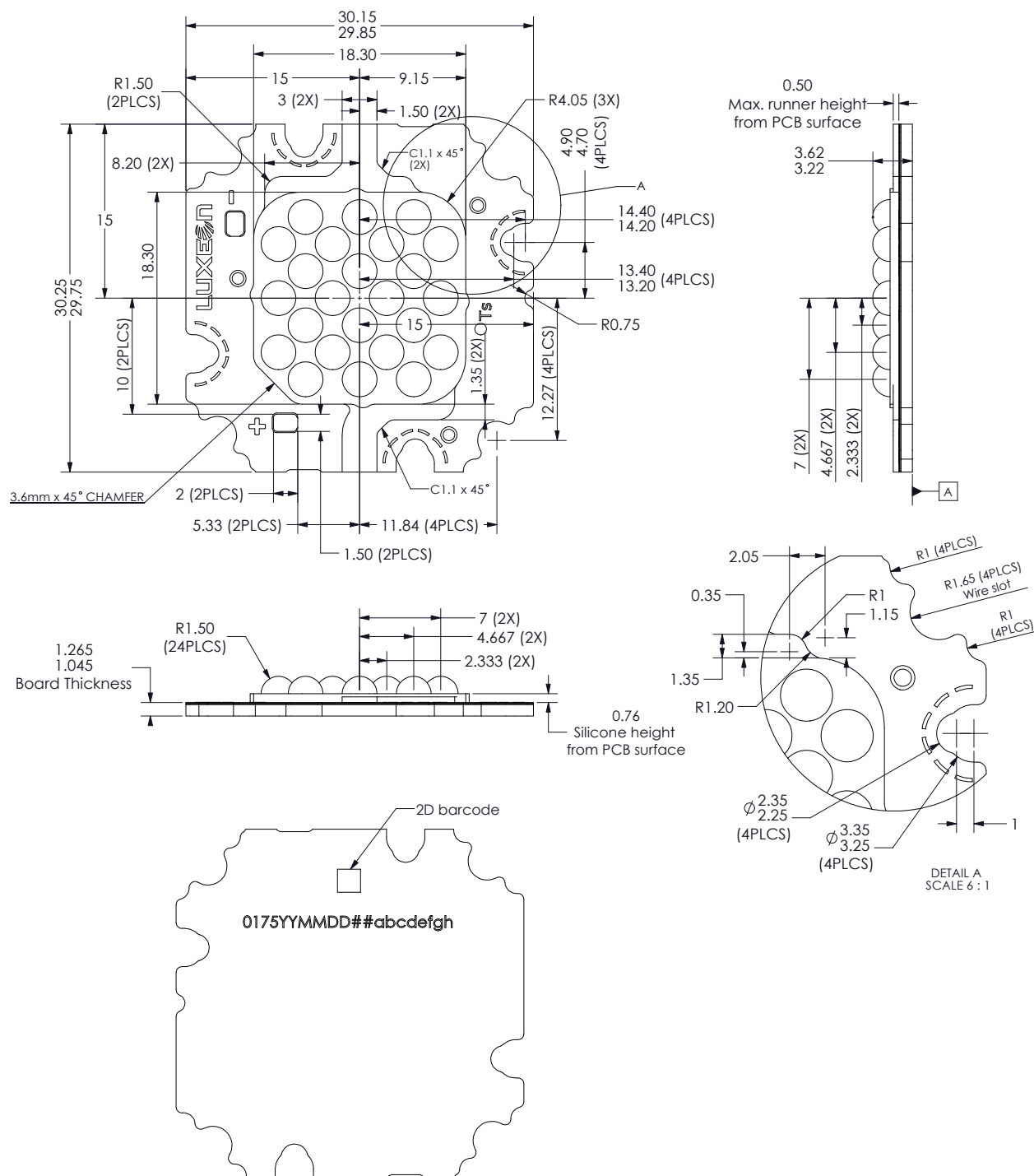
Figure 7. Dimensions for LKx-Pxxx-xx24(A).
