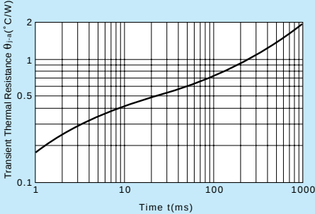
θj-a-t Characteristics
