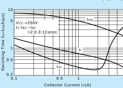
ton•tstg•tr-IC Characteristics (Typical)
