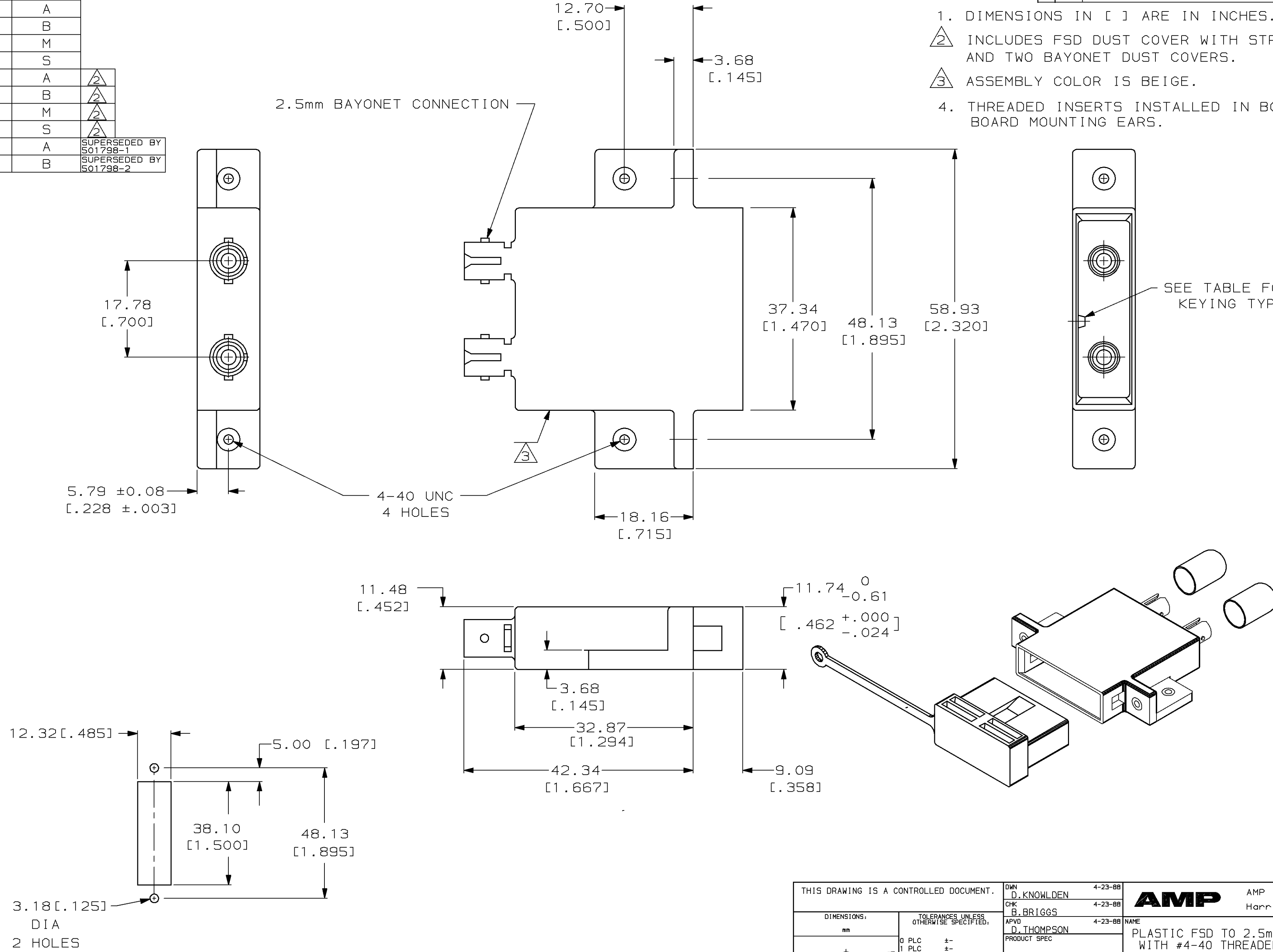
SUGGESTED MOUNTING PATTERN
