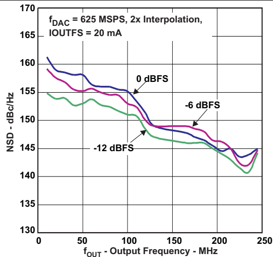
Figure 13. NSD vs Input Scale
