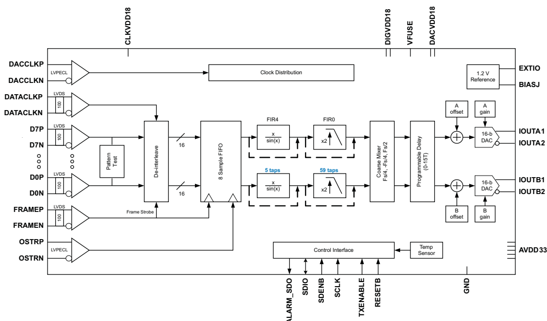
Simplified Schematic
