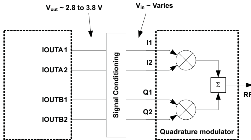
Figure 80. DAC to Analog Quadrature Modulator Interface
