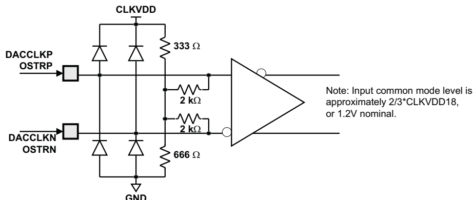
Figure 35. DACCLKP/N and OSTRP/N Equivalent Input Circuit
