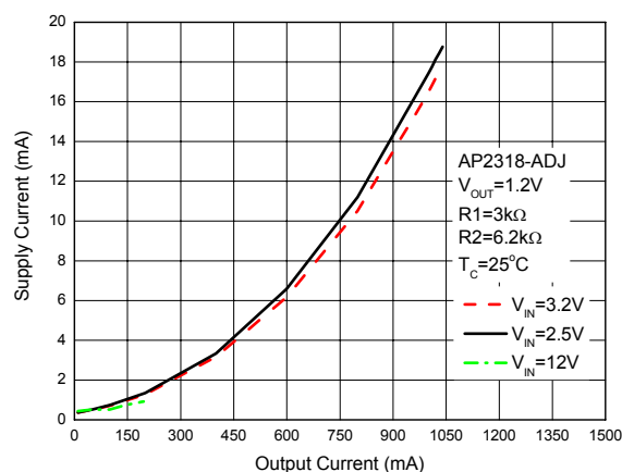
Figure 21. Supply Current vs. Output Current (Conditions: V_{OUT}=1.2V , R1=3k\Omega , R2=6.2k\Omega )
