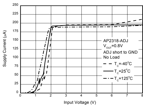
Figure 14. Supply Voltage vs. Input Voltage (Conditions: V_{OUT}=0.8V , ADJ Short to GND)
