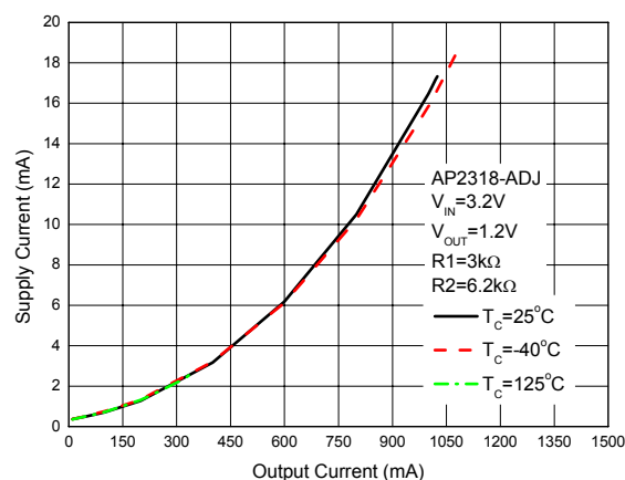
Figure 19. Supply Current vs. Output Current (Conditions: V_{\text{OUT}}=1.2\text{V} , R_1=3\text{k}\Omega , R_2=6.2\text{k}\Omega )
