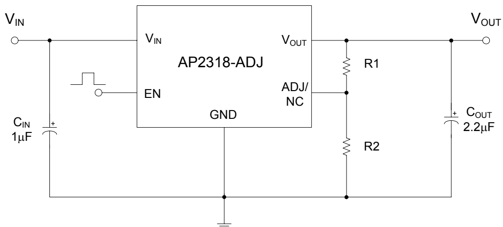
Figure 30. Typical Applications of AP2318 ADJ Version, V_{OUT}=0.8 \cdot (R1+R2)/R2
