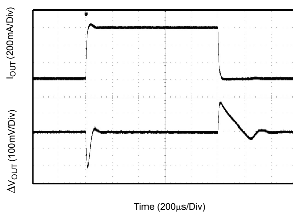
Figure 23. Load Transient Response (Conditions: V_{IN}=2.5V , V_{OUT}=1.8V , I_{OUT}=1mA to 600mA , C_{IN}=1\mu F , C_{OUT}=2.2\mu F )
