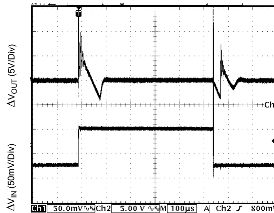
Figure 25. Line Transient Response (Conditions: V_{IN}=2.5V to 10V , V_{OUT}=0.8V , I_{OUT}=10mA , C_{IN}=0\mu F , C_{OUT}=2.2\mu F )
