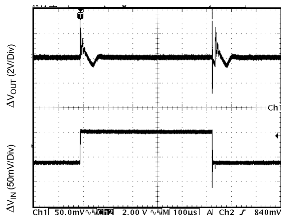
Figure 24. Line Transient Response (Conditions: V_{IN}=2.5V to 5V , V_{OUT}=0.8V , I_{OUT}=10mA , C_{IN}=0\mu F , C_{OUT}=2.2\mu F )
