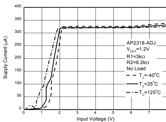
Figure 15. Supply Voltage vs. Input Voltage (Conditions: V_{OUT}=1.2V , R1=3k\Omega , R2=6.2k\Omega )
