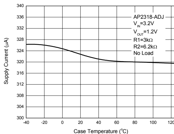
Figure 17. Supply current vs. Case Temperature (Conditions: V_{\text{OUT}}=1.2\text{V} , R_1=3\text{k}\Omega , R_2=6.2\text{k}\Omega )
