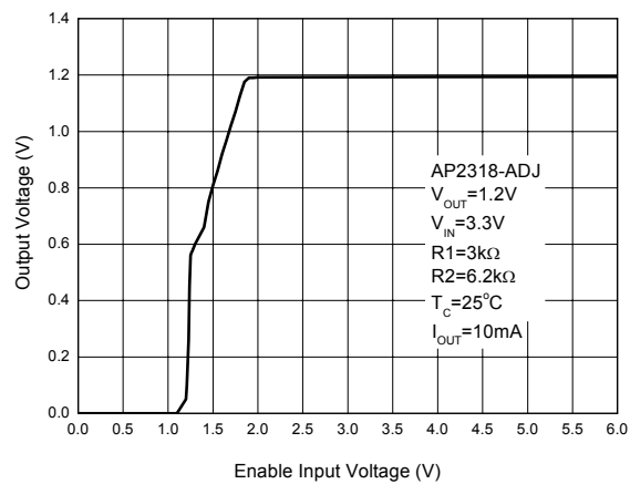
Figure 29. Output Voltage vs. Enable Input Voltage (Conditions: V_{OUT}=1.2V , R1=3k\Omega , R2=6.2k\Omega )
