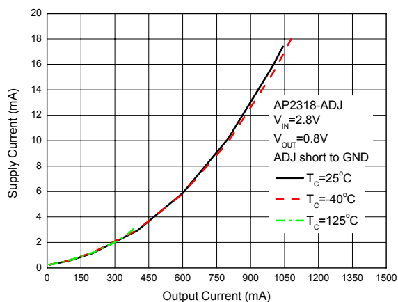
Figure 18. Supply Current vs. Output Current (Conditions: V_{\text{OUT}}=0.8\text{V} , ADJ Short to GND)
