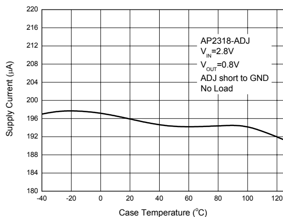
Figure 16. Supply Current vs. Case Temperature (Conditions: V_{\text{OUT}}=0.8\text{V} , ADJ Short to GND)
