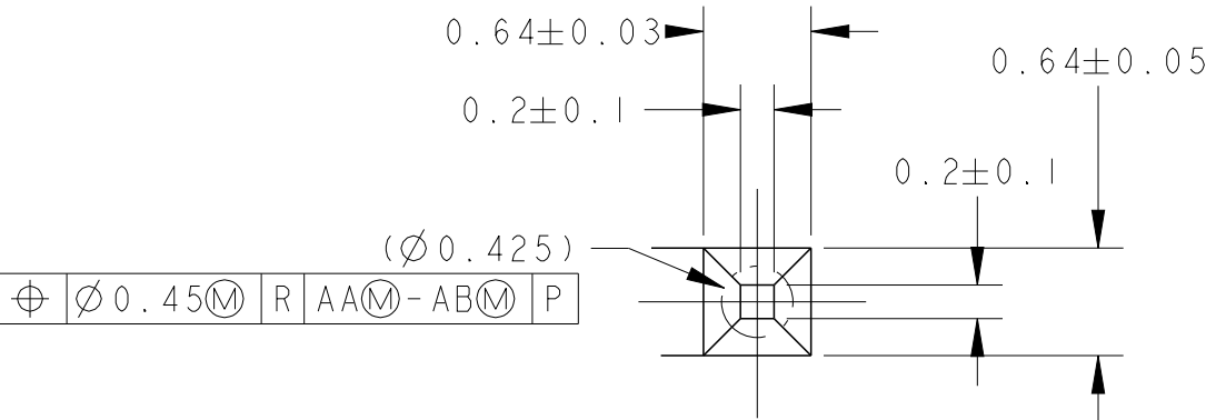
DETAIL B SCALE 20:1
