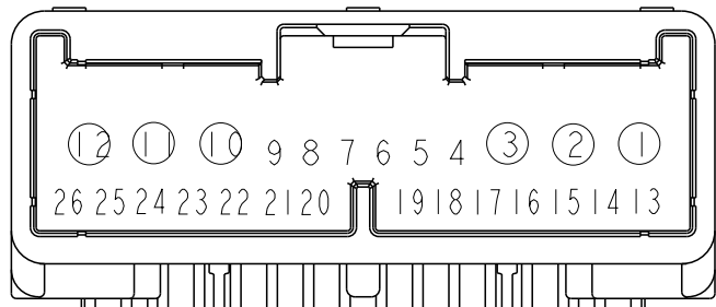
FIG. 1 CIRCUIT NUMBERS
