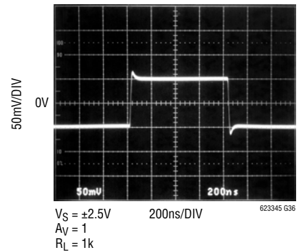
Small-Signal Response
