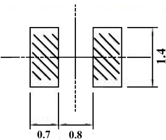
RECOMMENDED LANDING PATTERN
