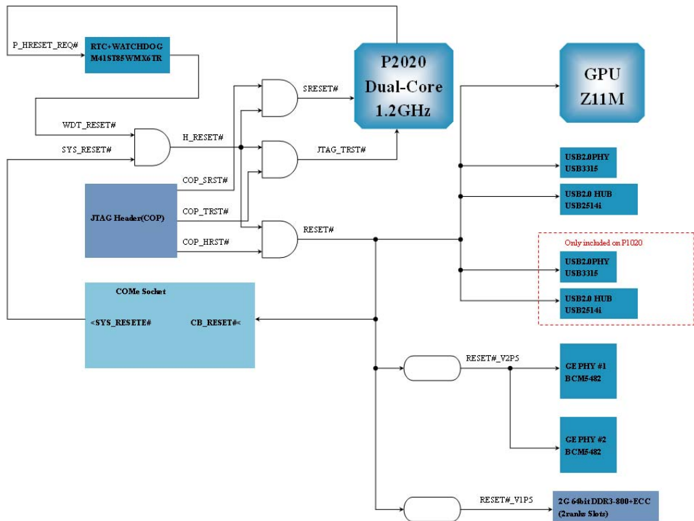
Figure 4-4 Reset Logic
