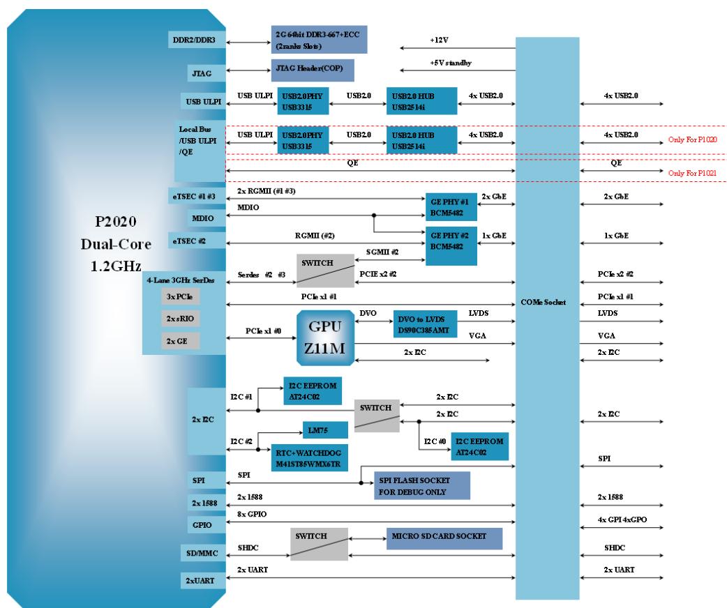
Figure 4-1 Block Diagram
