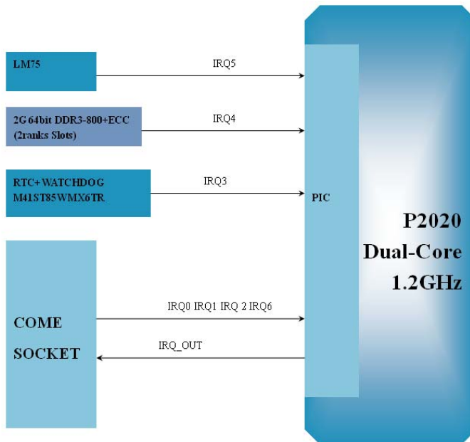
Figure 4-5 Interrupt Logic
