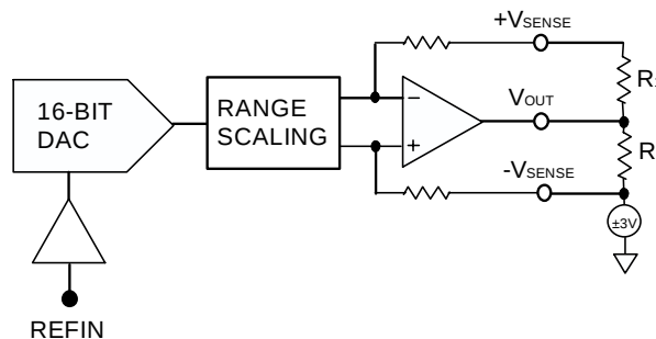
Figure 59. Voltage Output
