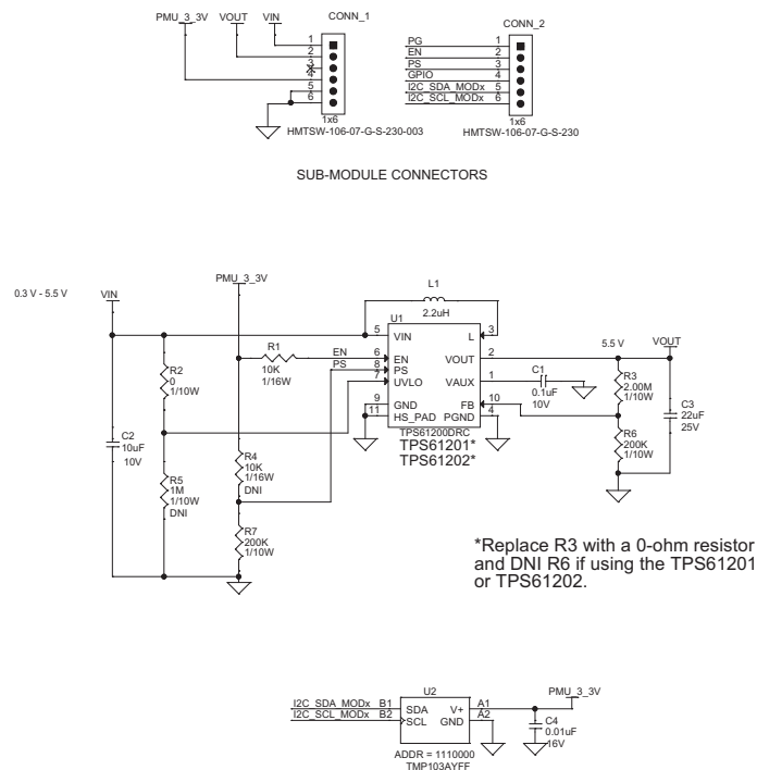
Figure 12. SMP-TPS61202-MVK Schematic
