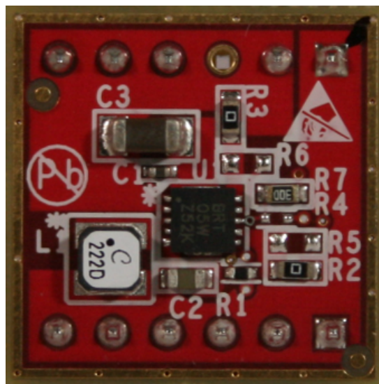
Figure 1. SMP-TPS61202-MVK Submodule
