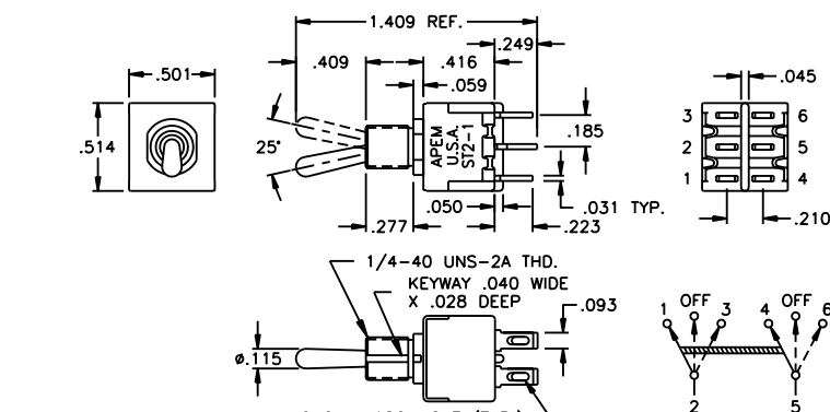
DOUBLE POLE
