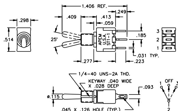
SINGLE POLE
