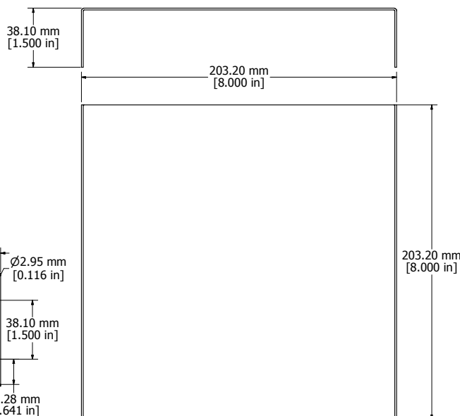
BOTTOM/TOP ENCLOSURE
