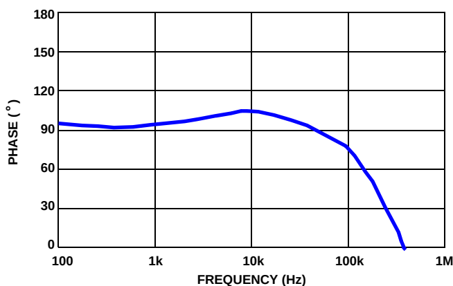
FIGURE 52. SIMULATED LOOP GAIN
