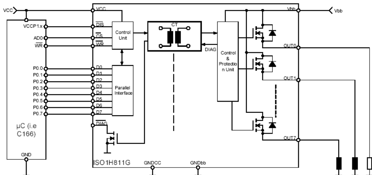
Typical Application
