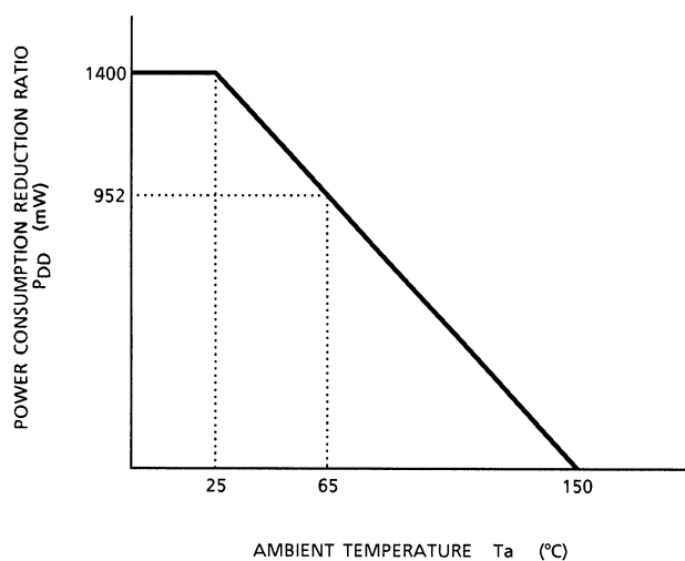
(a) TA1287P
