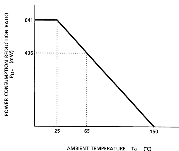
(b) TA1287FG
