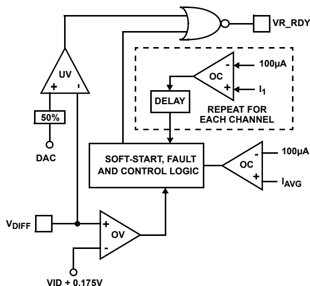
FIGURE 12. VR_RDY AND PROTECTION CIRCUITRY
