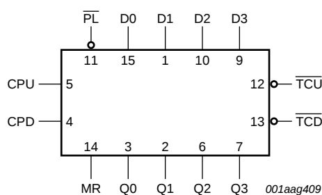
Fig 2. Logic symbol
